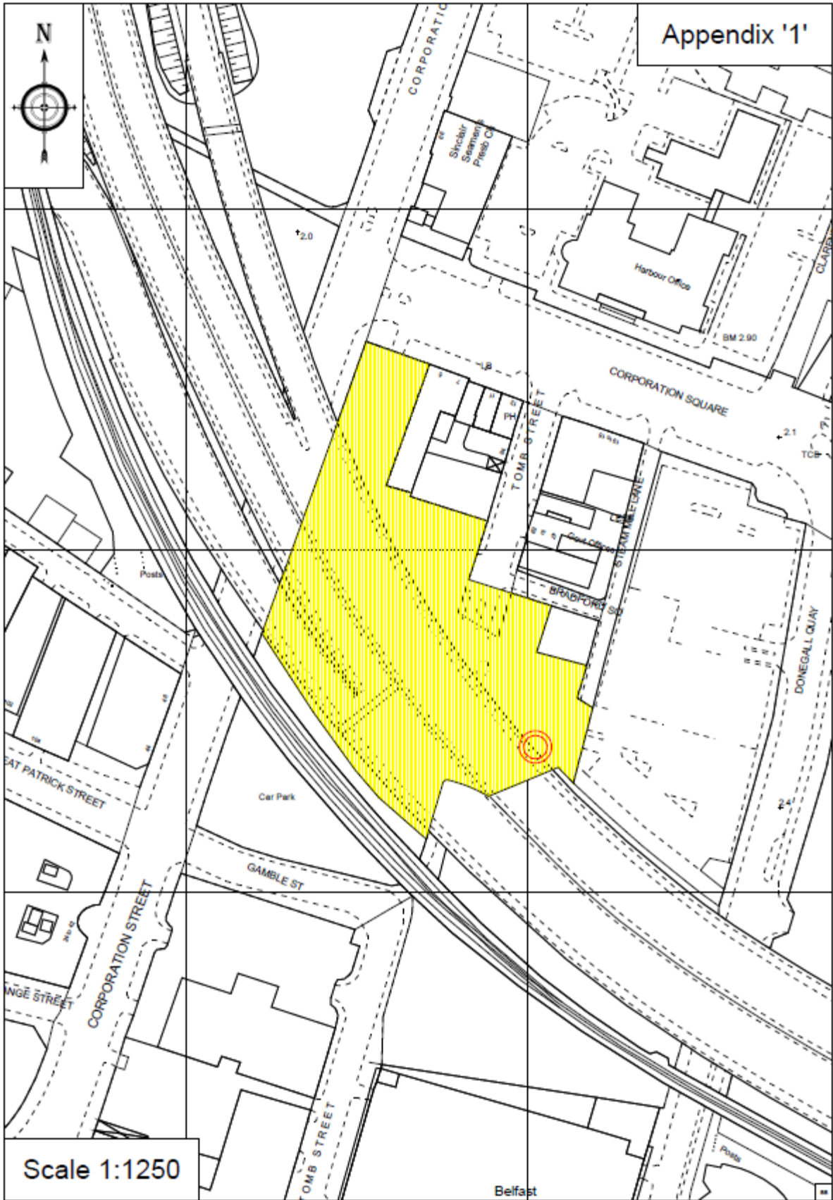
Proposed location of reception shaft
